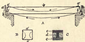
FIG. 37. Principle of the girder.
